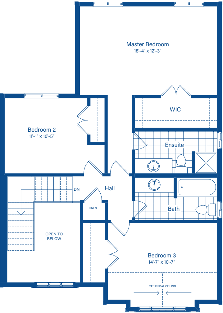
2ND FLOOR
